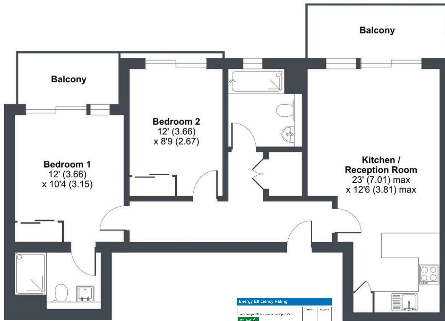
FIRST FLOOR
